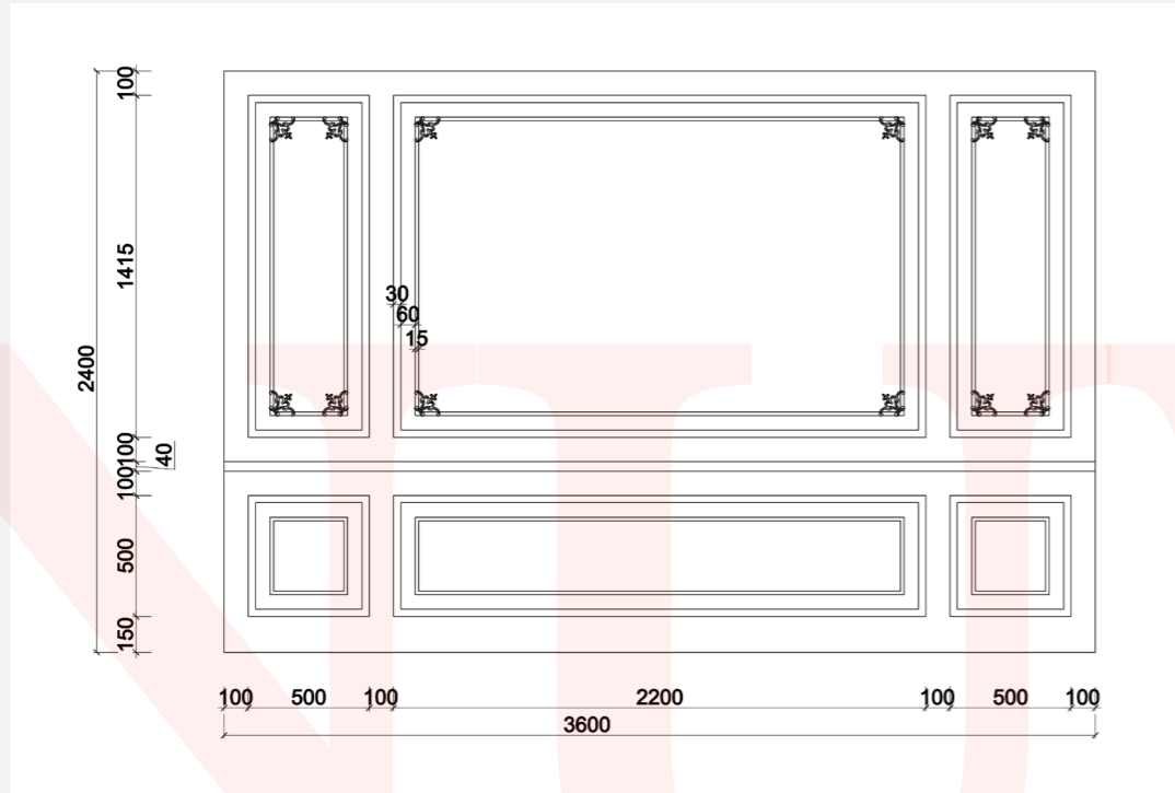
PU mouldings double frame structure Double frame structure
