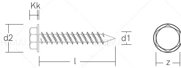
Hex Washer Head Self Tapping Screw
